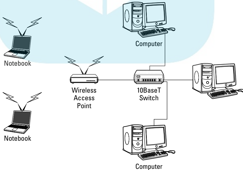
Figure 9-3: A wireless access point connects a wireless network to a cabled network.
